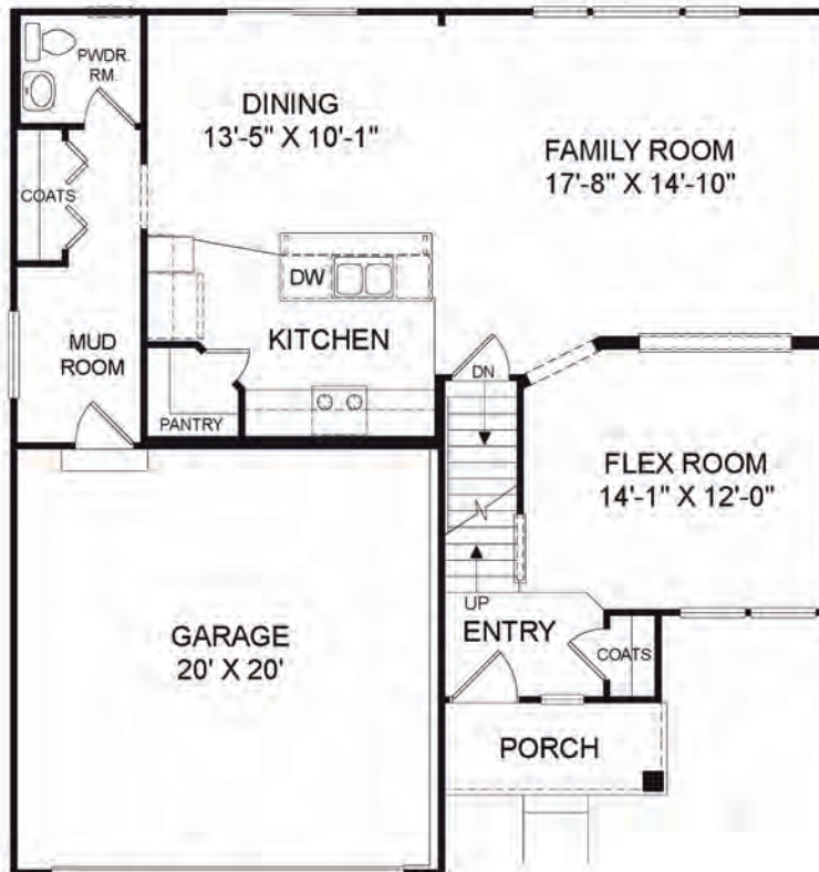
FIRST FLOOR 8' CEILING HT. DIMENSIONS 38'W x 40'D 2008 SF TOTAL
